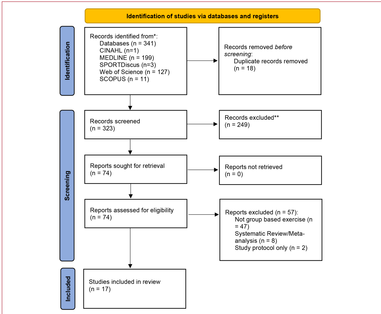
Figure 1. PRISMA flowchart.
